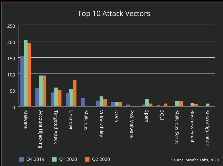
FIGURE 6. OVERALL, MALWARE LED DISCLOSED ATTACK VECTORS IN THE SECOND QUARTER OF 2020, ACCOUNTING FOR 35% OF PUBLICLY REPORTED INCIDENTS. ACCOUNT HIJACKING ATTACKS FOLLOWED TOTALING 17%, AND TARGETED ATTACKS 9%.
